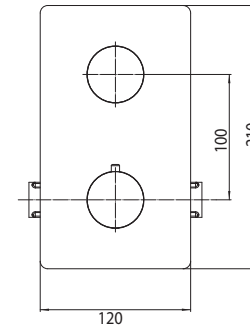
INZ001 MISCELATORE TERMOSTATICO 2-3-4-5 USCITE THERMOSTATIC MIXERS 2-3-4-5 OUTLETS
