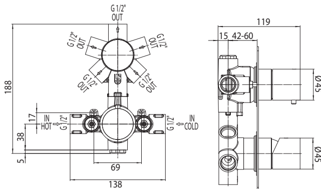
INZ001 MISCELATORE TERMOSTATICO 2-3-4-5 USCITE THERMOSTATIC MIXERS 2-3-4-5 OUTLETS
